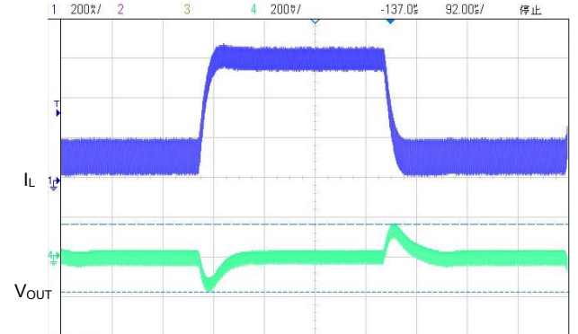
(16) Load Transient(VIN=50.0V,VOUT=12V,IOUT=0.1→0.6A)
