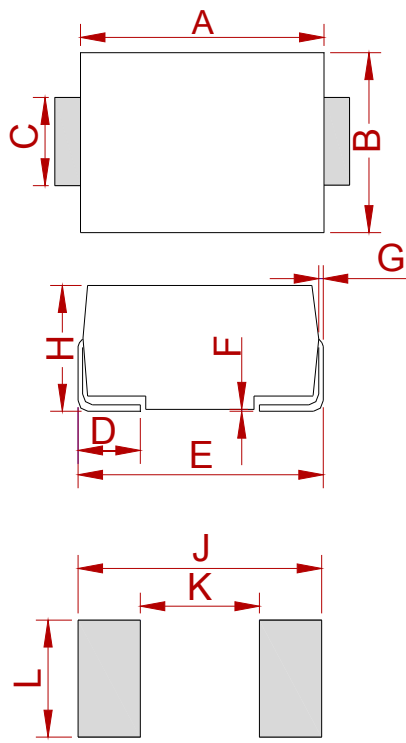
DO-214AA (SMB)
