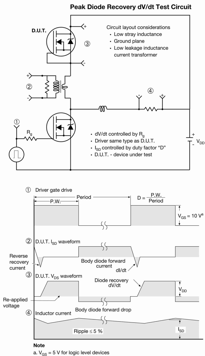
Fig. 19 - For N-Channel
