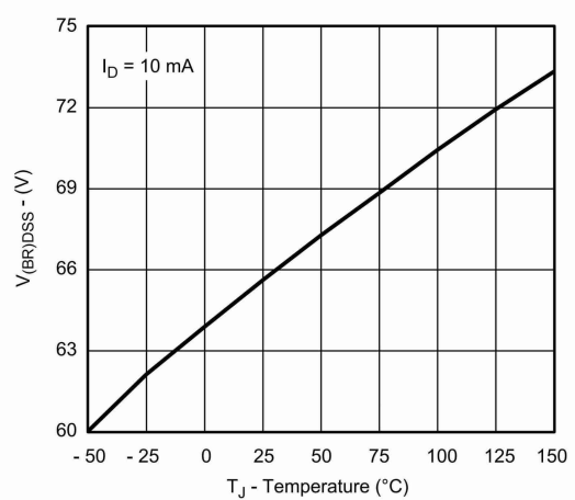
Drain-Source Breakdown Voltage vs. Junction Temperature
