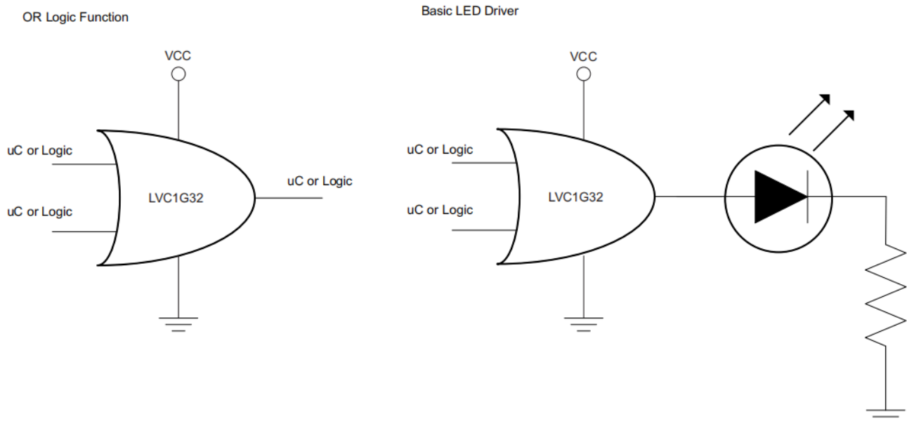
Figure 5.1: Application Schematic
