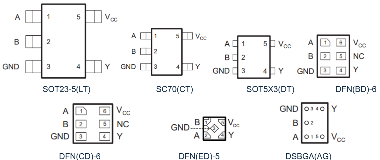
Figure 2.1 Top View
