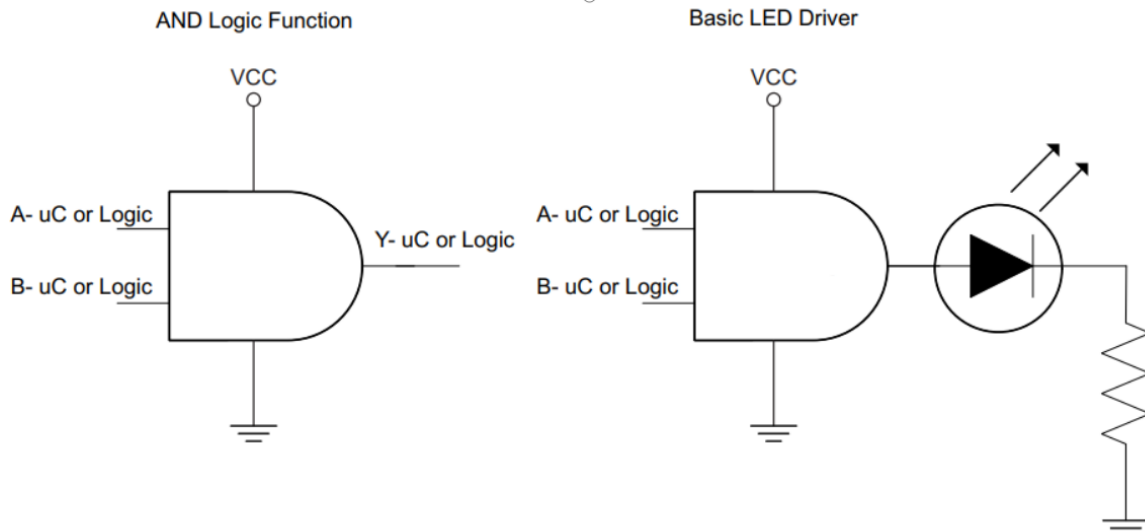
Figure 5.1: Application Schematic
