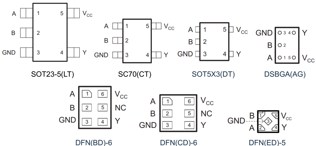
Figure 2.1: Top View
