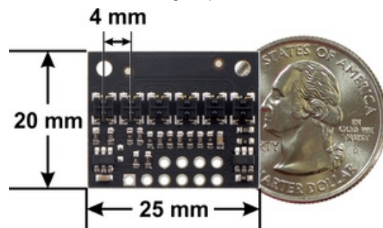
QTRX-HD-06A Reflectance Sensor Array dimensions.
