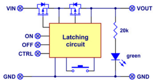
Block diagram of the Big Pushbutton Power Switch with Reverse Voltage Protection.
