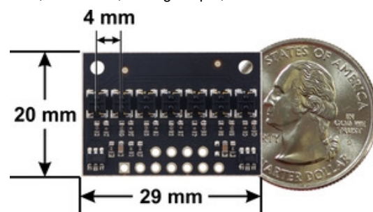
QTRX-HD-07A Reflectance Sensor Array dimensions.
