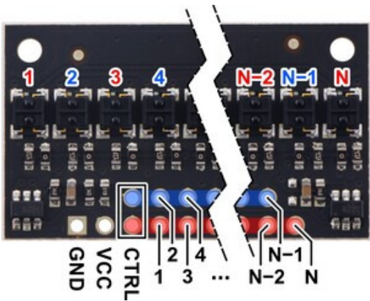
Pinout diagram of a QTRX-HD-xA Reflectance Sensor Array.
