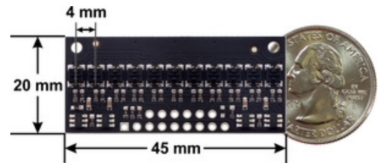
QTRX-HD-11A Reflectance Sensor Array dimensions.
