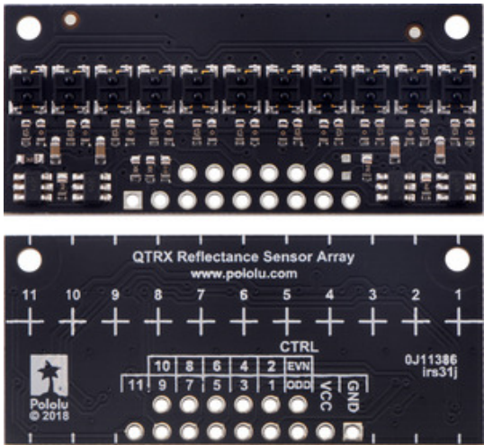
QTRX-HD-11A Reflectance Sensor Array, front and back views.
