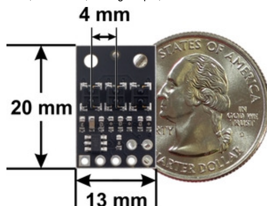
QTRX-HD-03A Reflectance Sensor Array dimensions.
