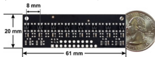
QTR-MD-08RC Reflectance Sensor Array dimensions.
