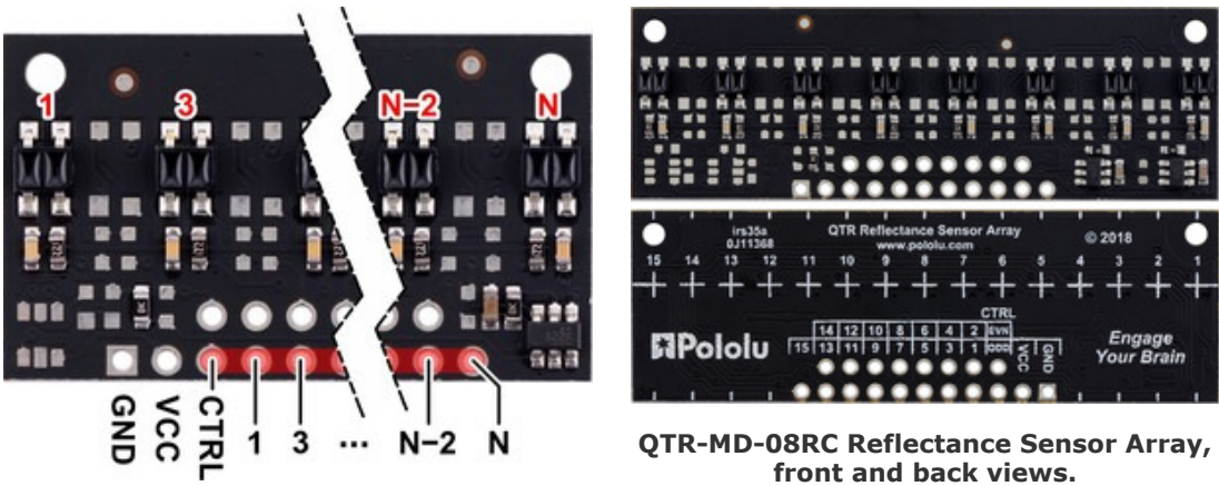
Pinout diagram of a QTR-MD-xRC Reflectance Sensor Array.
