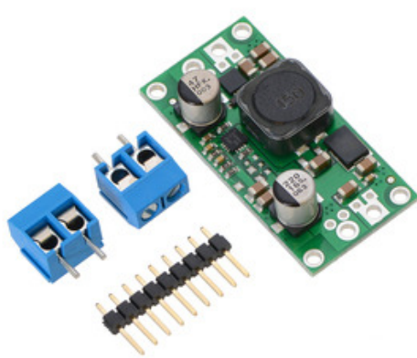
Pololu fixed step-up/step-down voltage regulator S18V20Fx with included optional terminal blocks and header pins.
