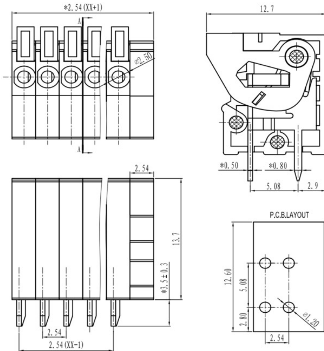
Screwless terminal block: 0.1" pitch, top entry.
