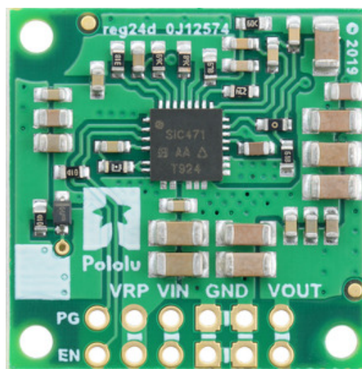
7.5V, 5A Step-Down Voltage Regulator D36V50F7, bottom view.
