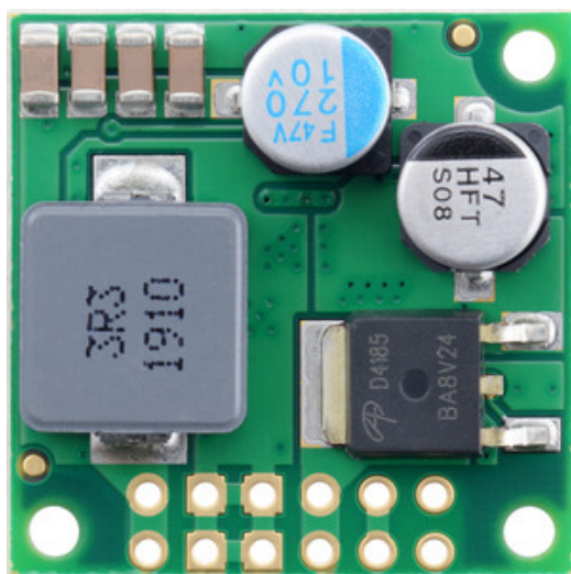
7.5V, 5A Step-Down Voltage Regulator D36V50F7, top view.
