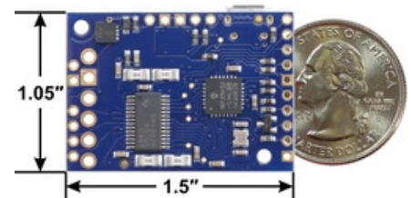
Tic T825 USB Multi-Interface Stepper Motor Controller, bottom view with dimensions.
