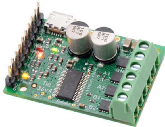
Tic 36v4 USB Multi-Interface High-Power Stepper Motor Controller (Connectors Soldered).
