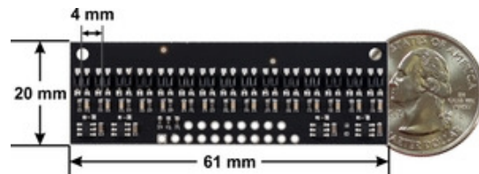
QTR-HD-15RC Reflectance Sensor Array dimensions.
