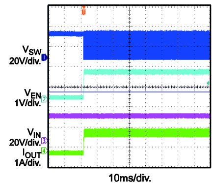
V_{EN} Startup
