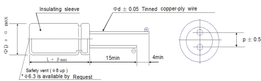
寸法图DIMENSIONS
