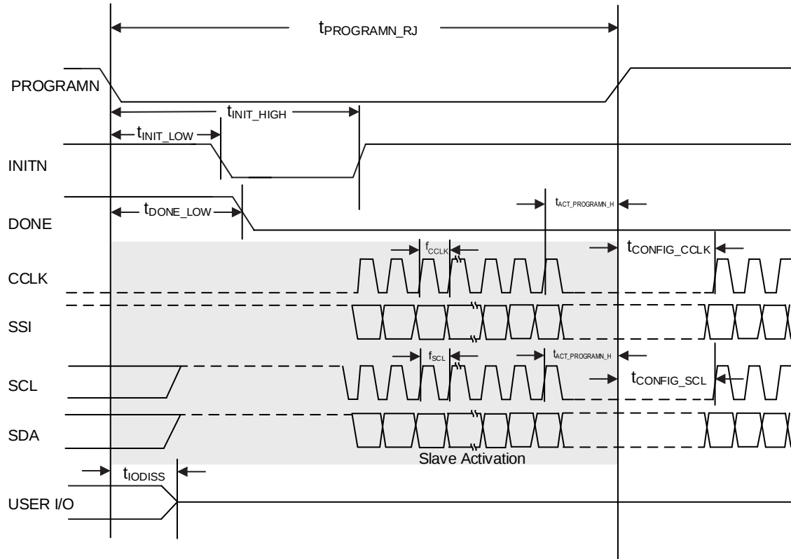
Figure 4.18. Slave SPI/I²C/I³C PROGRAMN Timing
