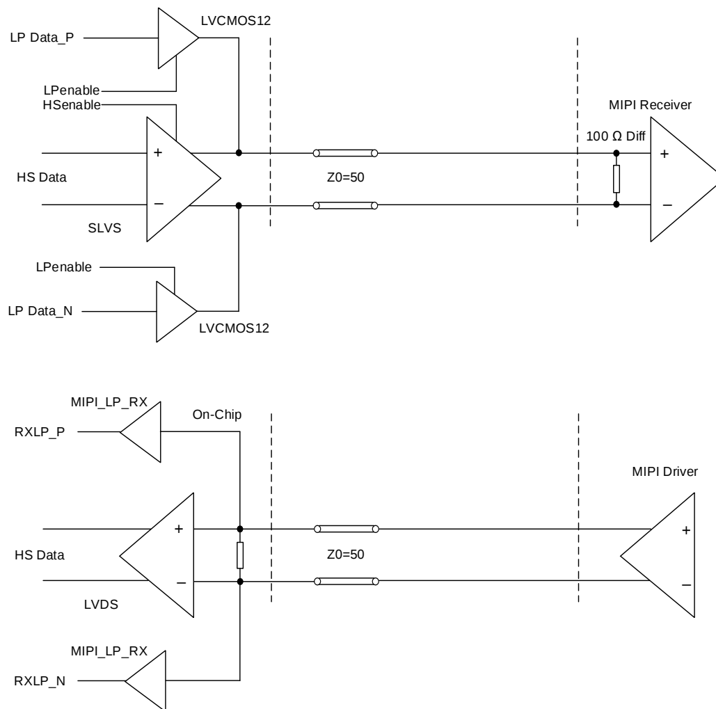
Figure 4.6. MIPI Interface
