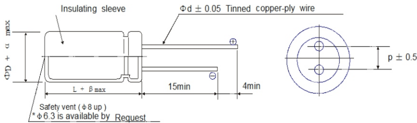
寸法图DIMENSIONS
