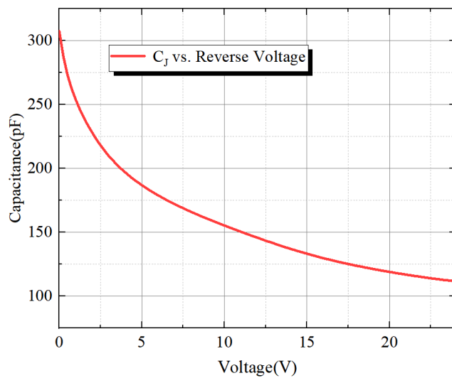
Capacitance vs. vs. Reverse Voltage
