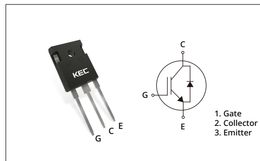
PIN CONFIGURATION
