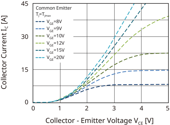
Fig3. Typical Output Characteristic ( I_C vs V_{CE} )@ T_J=T_{Jmax}
