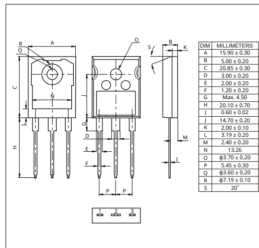
PACKAGE DIMENSION(TO-247)
