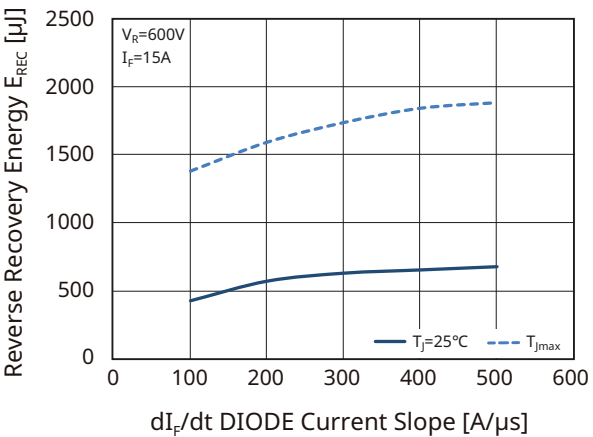
Fig22. Typical Reverse Recovery Energy as a Function of DIODE Current Slope
