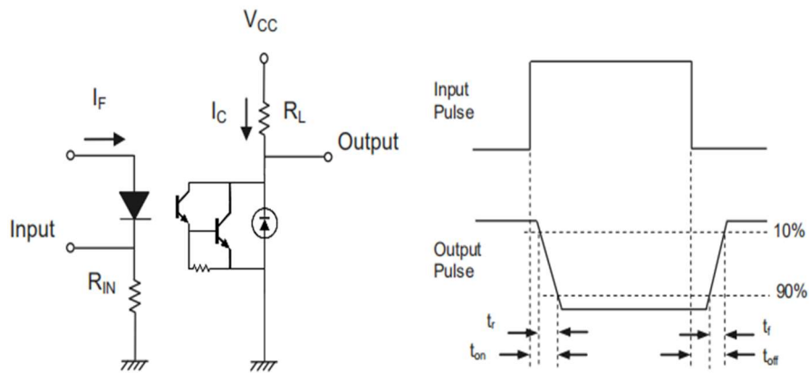
Fig.7 Test circuit diagram
