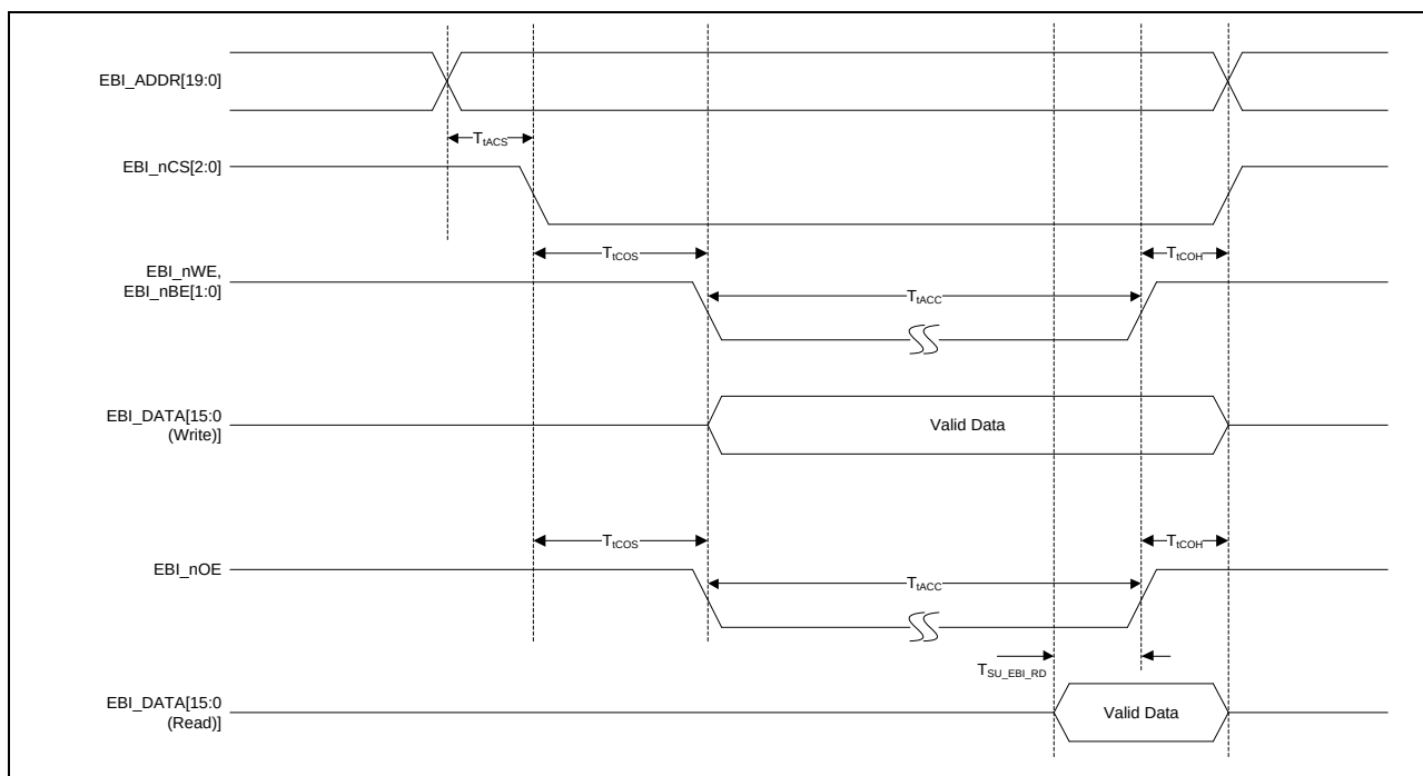
Figure 9.6-10 External Bus Interface Timing Diagram
