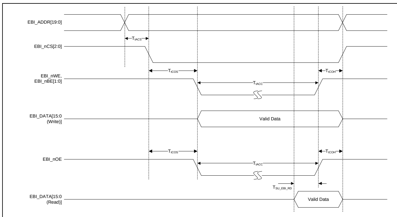
Figure 8.15-1 External Bus Interface Timing Diagram
