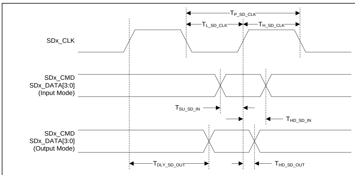
Figure 9.6-9 SDIO High-speed Mode
