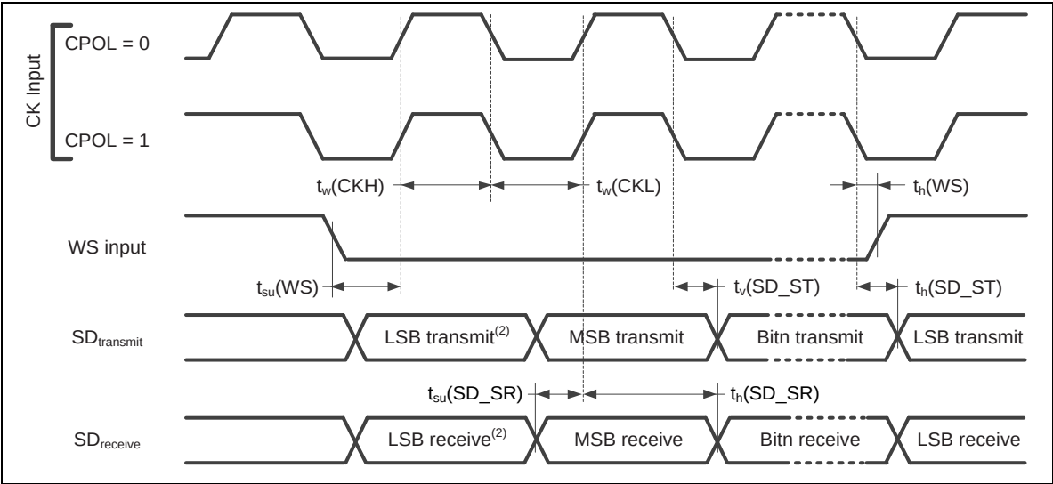
Figure 8.9-2 I²S Slave Mode Timing Diagram
