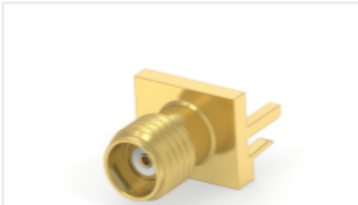
TE 产品编号2081880-1 EP-SMA,JACK,27GHZ,END LAUNCH, 1.5MM BOARD
