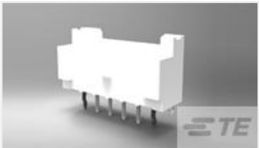
TE 产品编号2132230-7 EP2.5 Shrouded HDR ASSY 7P VER
