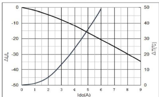
YSPI0740-6R8M
