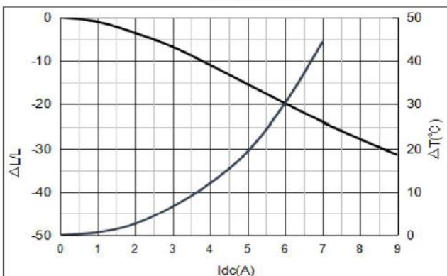
YSPI0740-4R7M
