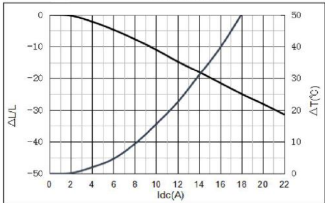
YSPI0740-1R5M
