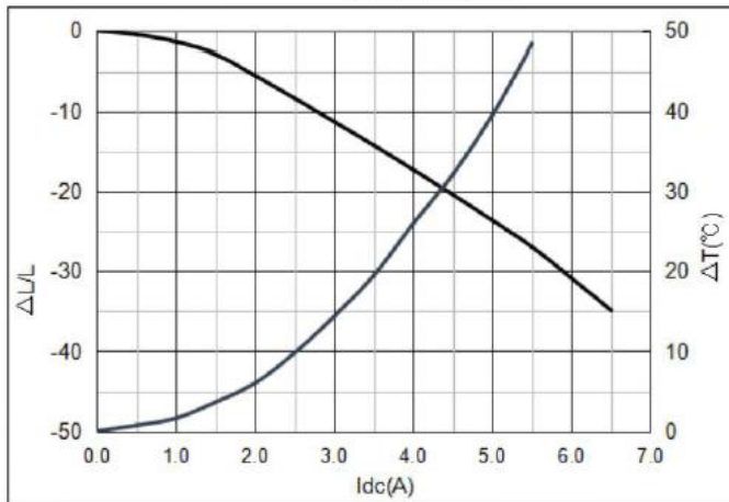
YSPI0740-220M
