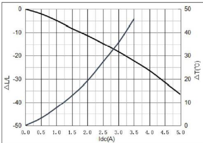
YSPI0740-220M
