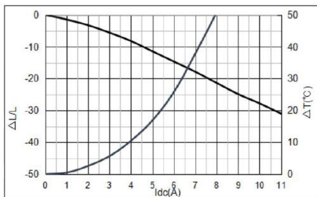
YSPI0740-6R8M
