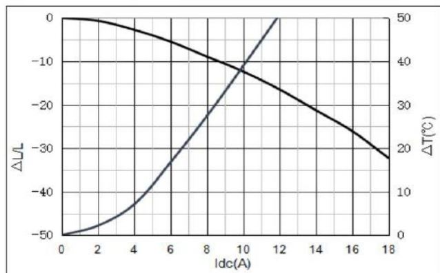
YSPI0740-3R3M
