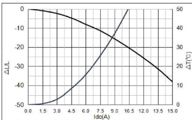
YSPI0740-4R7M
