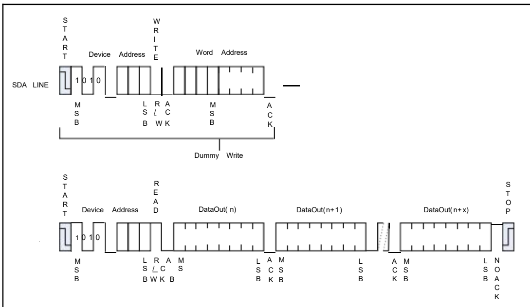
Figure 5-5 Sequential Read
