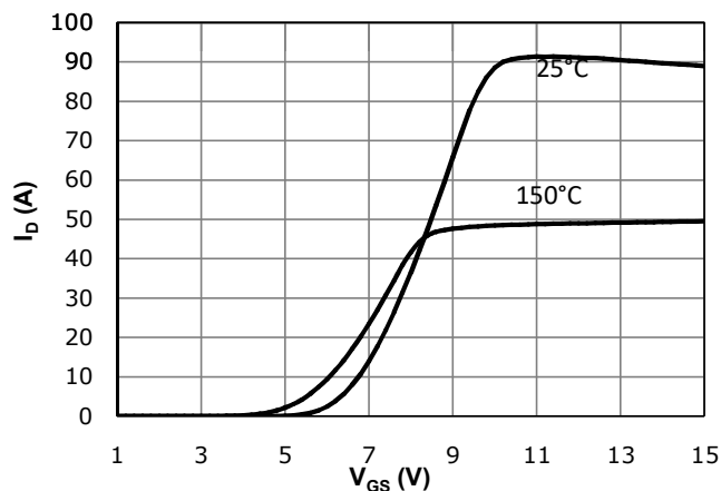
Fig 3: Transfer Characteristics
