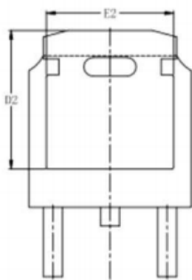
OPTION 2 BOTTOM VIEW
