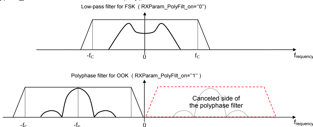
Figure 17: Active Channel Filter Description
