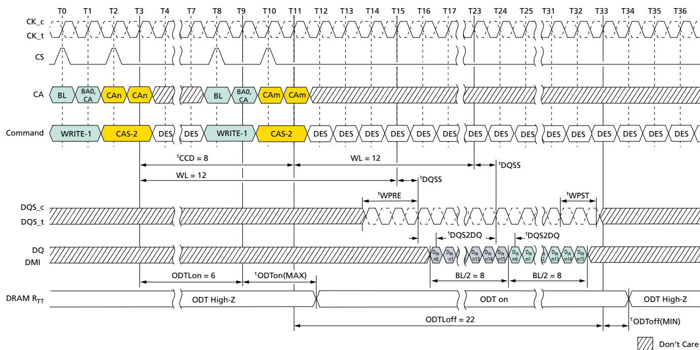
Figure 56: Seamless WRITE: t_{CCD} = \text{MIN} , 1.5nCK Postamble, 533 \text{ MHz} < \text{Clock Frequency} \leq 800 \text{ MHz} , ODT Worst Timing Case
