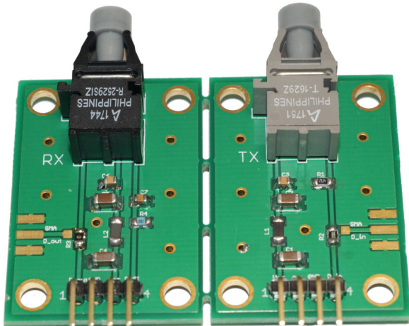
Figure 6: Modified Interfaces with SMA Connectors for Tx Input and Rx Output Signals
