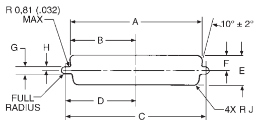
Standard Cutout
