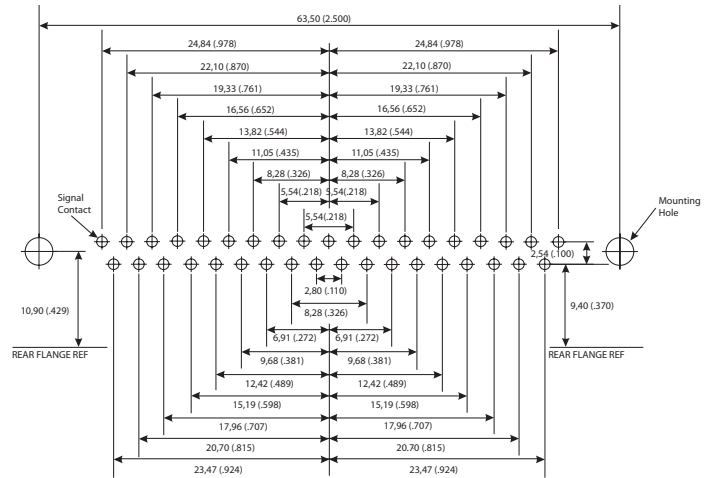
37 Contacts
