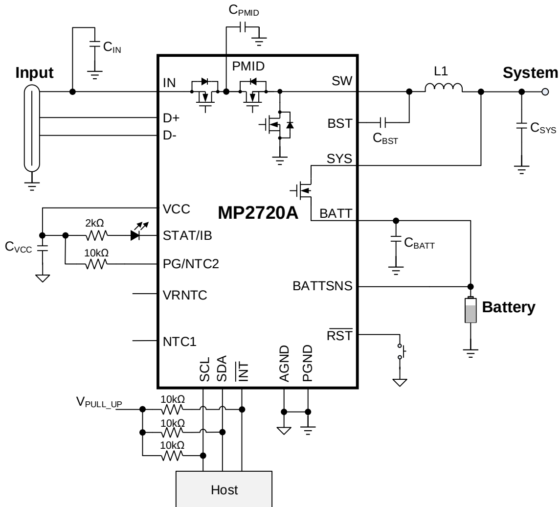
Figure 16: Typical Application Circuit
