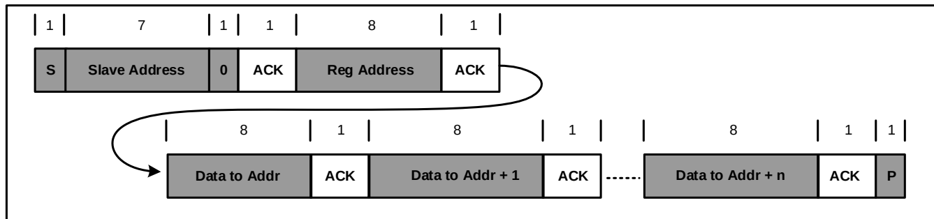
Figure 13: Multi-Write Sequence
