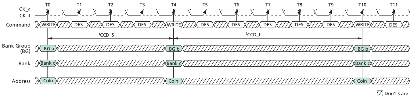
Figure 120: Write Burst t_{CCD\_S} and t_{CCD\_L} Examples
