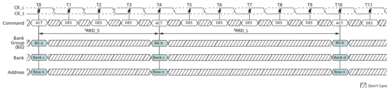
Figure 81: t_{RRD} Timing
