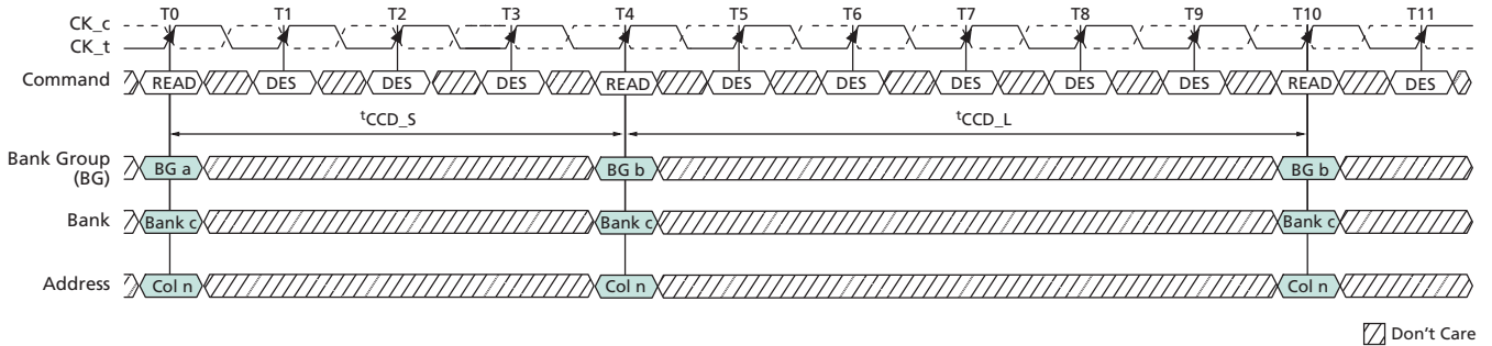
Figure 119: READ Burst t_{CCD\_S} and t_{CCD\_L} Examples
