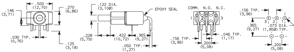
8121SD9A6GE SPDT
