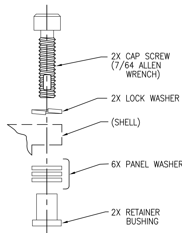
MTC50 HARDWARE APPLIES TO -020 MODIFICATION (see table I)
