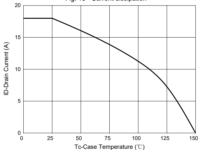
Fig. 10 - Current dissipation
