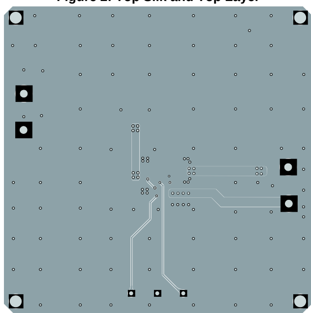
Figure 4: Inner2 Layer
