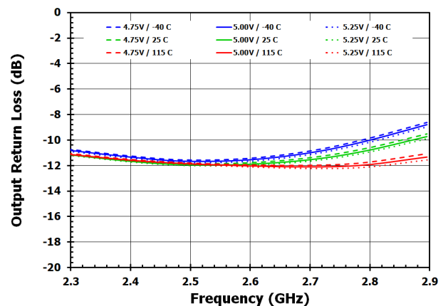
Figure 5. Output Return Loss
