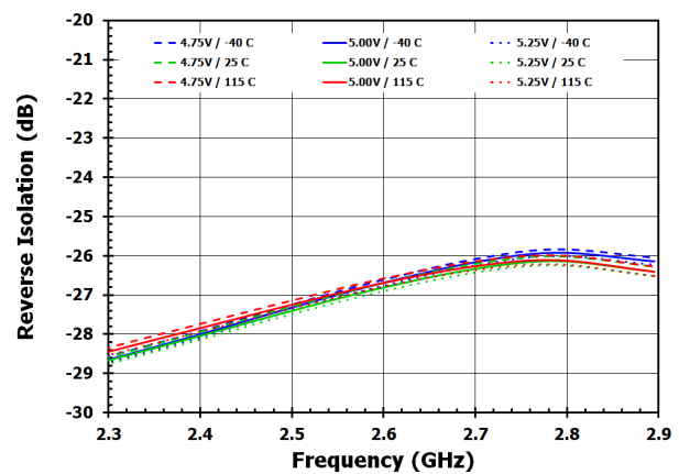
Figure 3. Reverse Isolation
