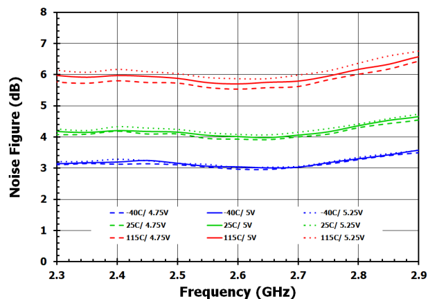
Figure 9. Noise Figure
