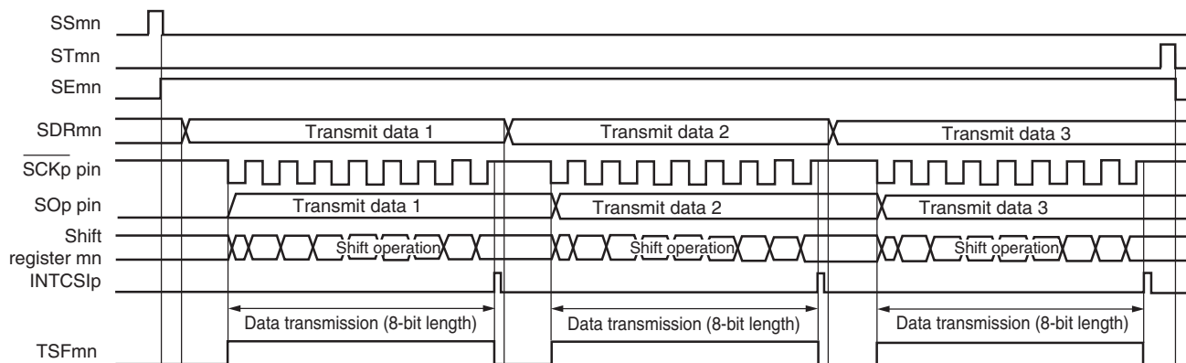
Figure 15-74. Timing Chart of Slave Transmission (in Single-Transmission Mode)
