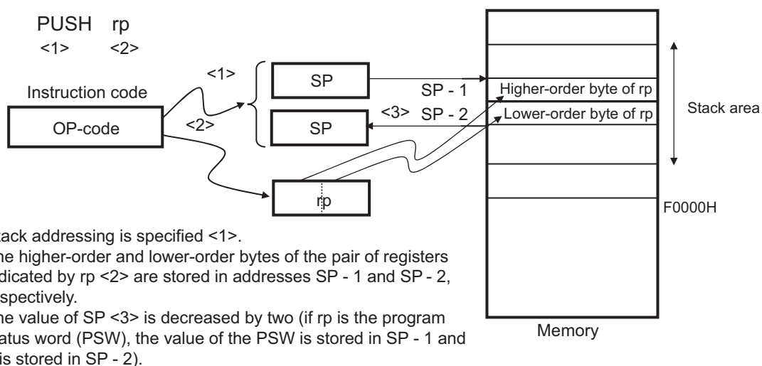
Figure 3-40. Example of PUSH rp
