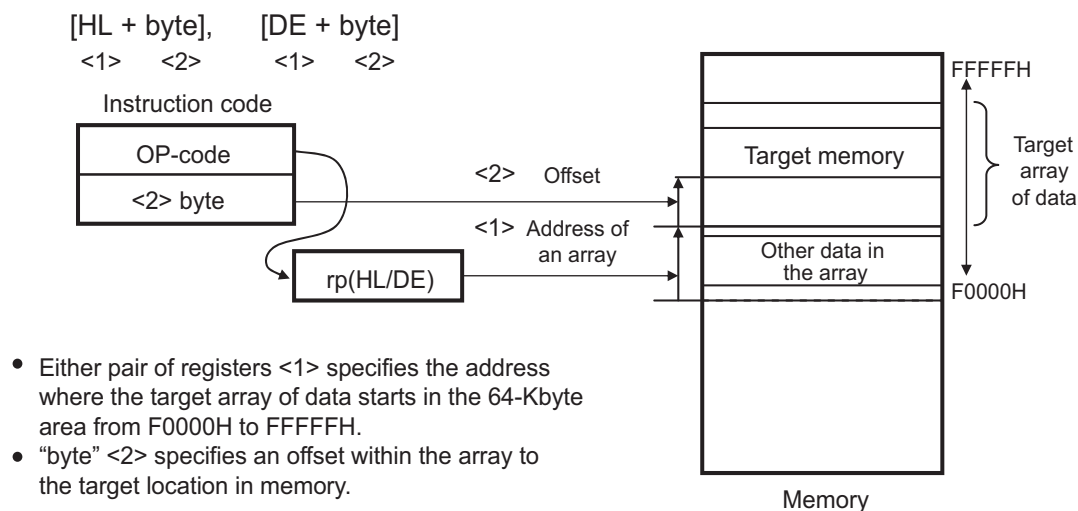
Figure 3-32. Example of [HL + byte], [DE + byte]
