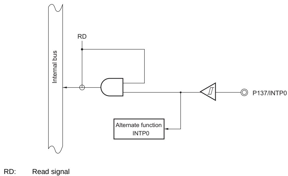
Figure 4-82. Block Diagram of P137
