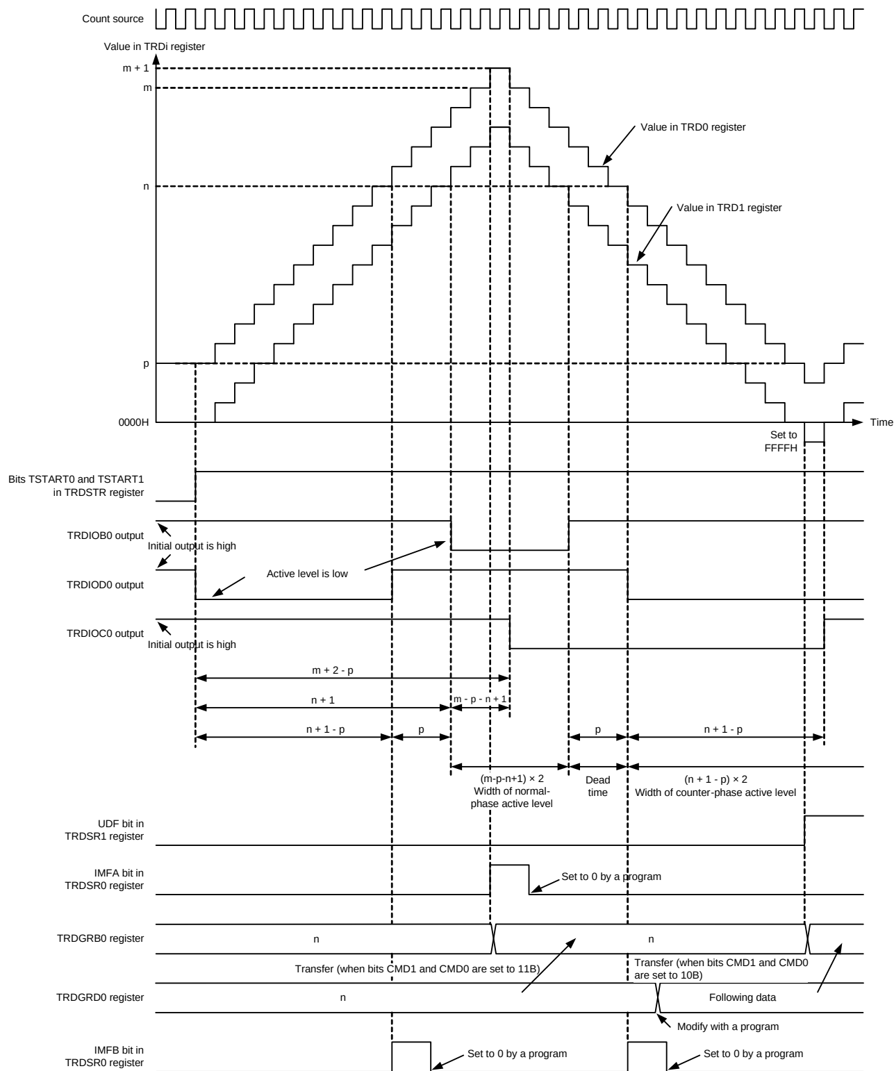
Figure 8-59. Operation Example in Complementary PWM Mode
