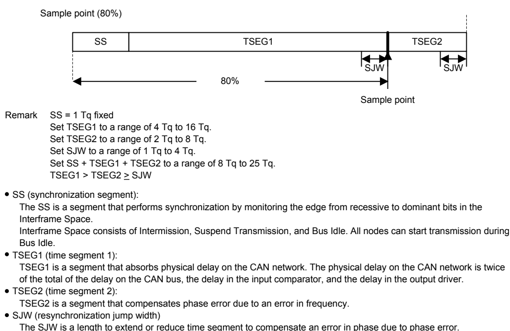
Figure 18-18. Bit Timing Chart
