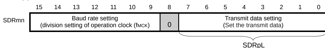
Figure 15-30. Example of Contents of Registers for Master Transmission of 3-Wire Serial I/O (CSI00, CSI01, CSI10, CSI11, CSI20, CSI21) (2/2)
