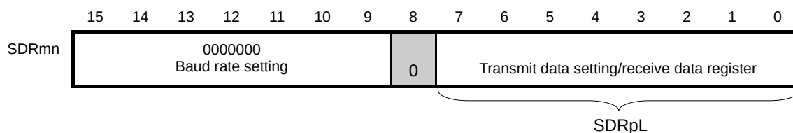
Figure 15-90. Example of Contents of Registers for Slave Transmission/Reception of 3-Wire Serial I/O (CSI00, CSI01, CSI10, CSI11, CSI20, CSI21) (2/2)
