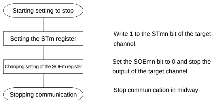
Figure 15-136. Procedure for Stopping Slave Transmission
