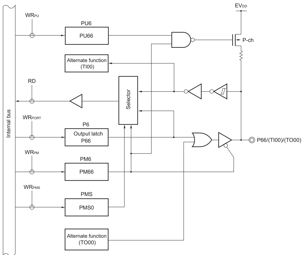
Figure 4-51. Block Diagram of P66
