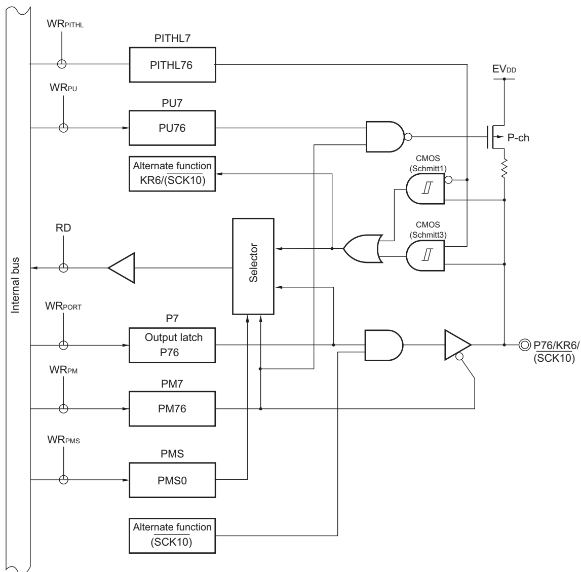
Figure 4-59. Block Diagram of P76
