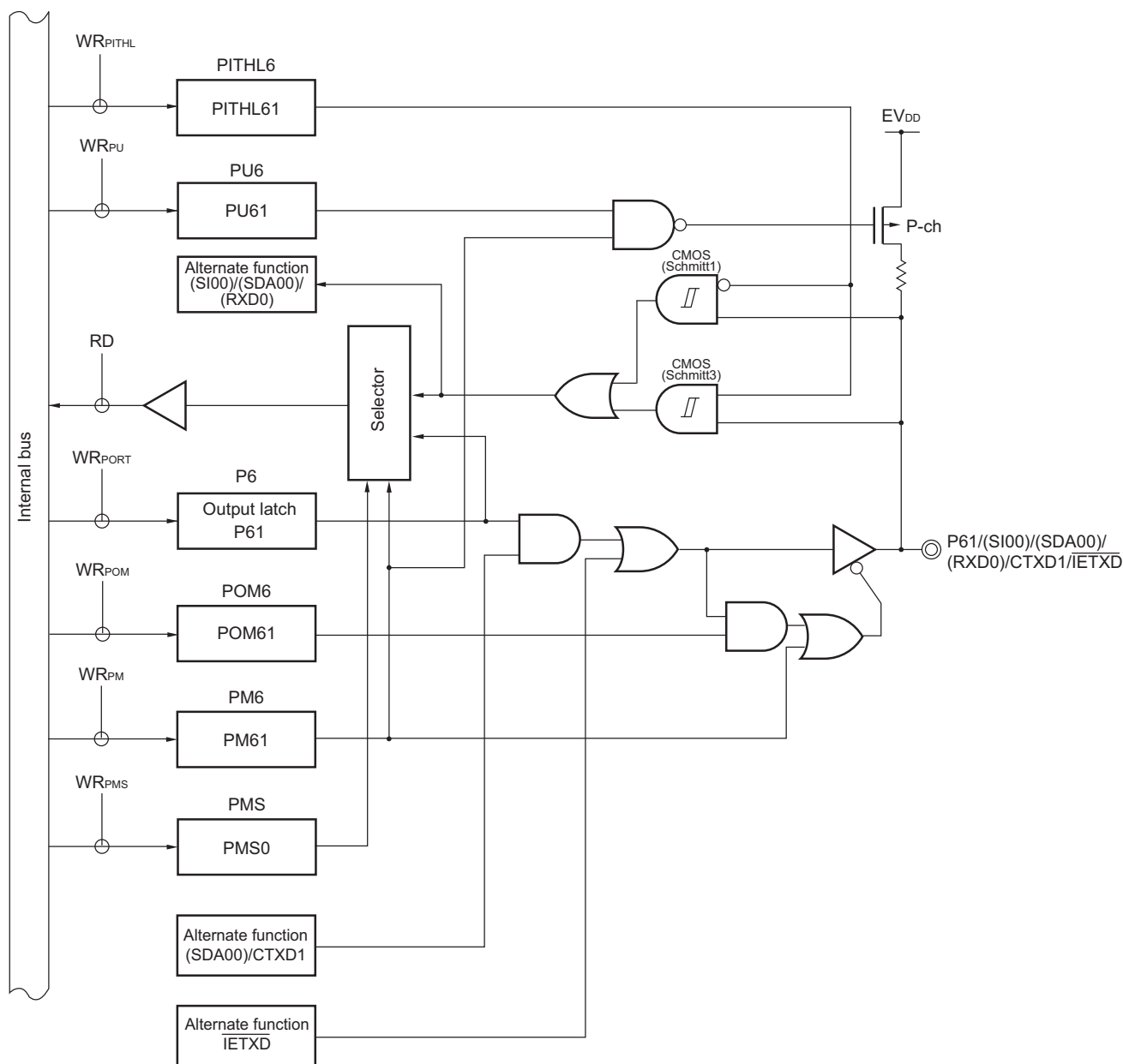
Figure 4-46. Block Diagram of P61
