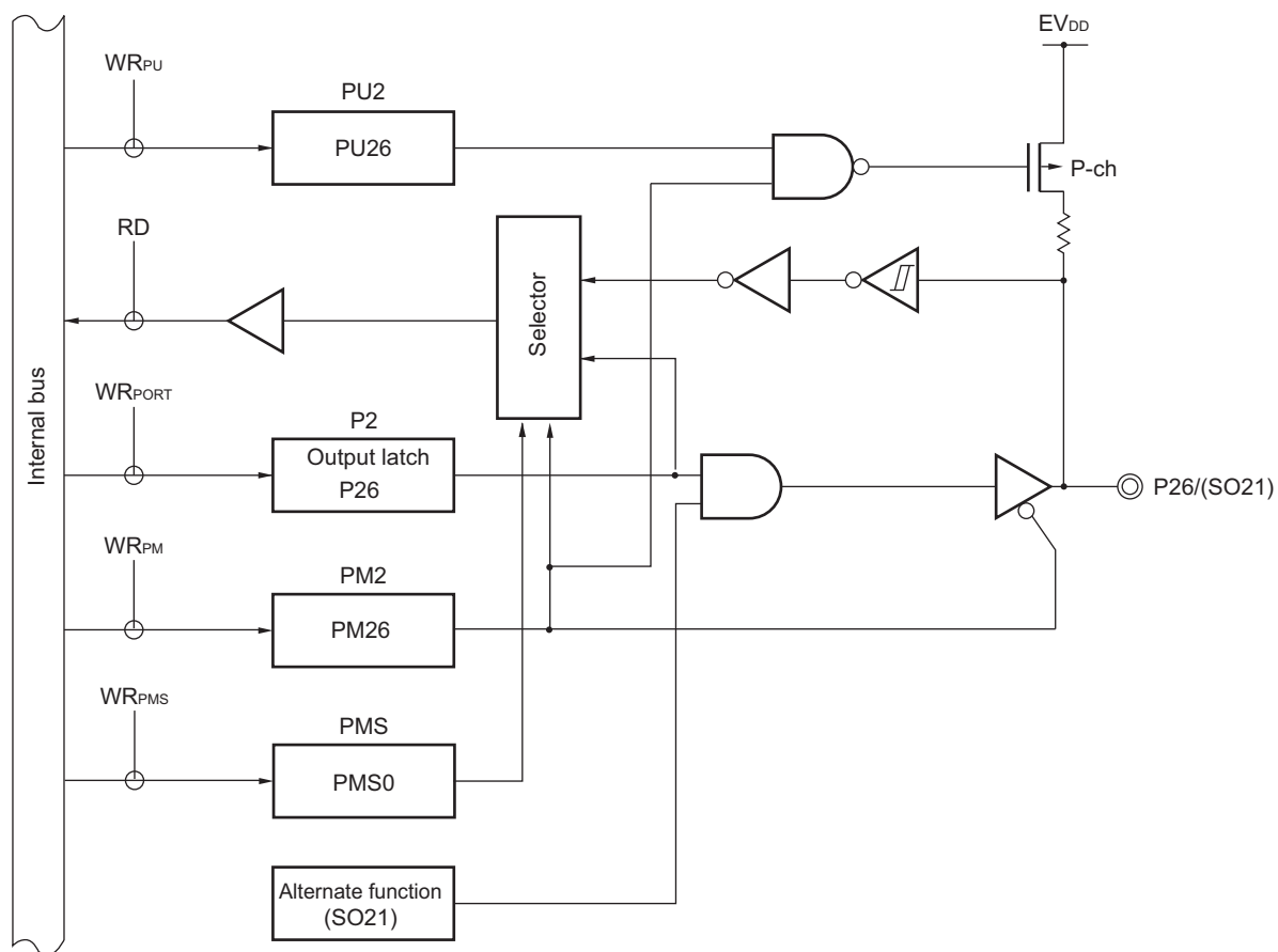
Figure 4-21. Block Diagram of P26
