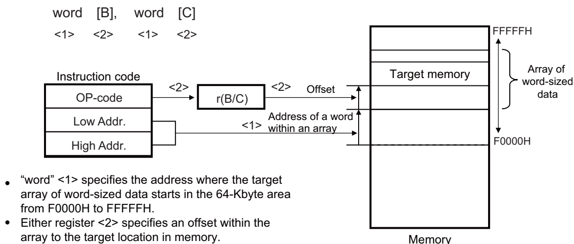
Figure 3-33. Example of word[B], word[C]
