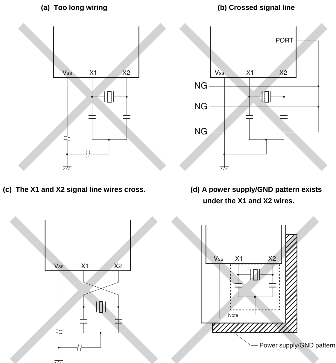
Figure 5-22. Examples of Incorrect Resonator Connection (1/2)
