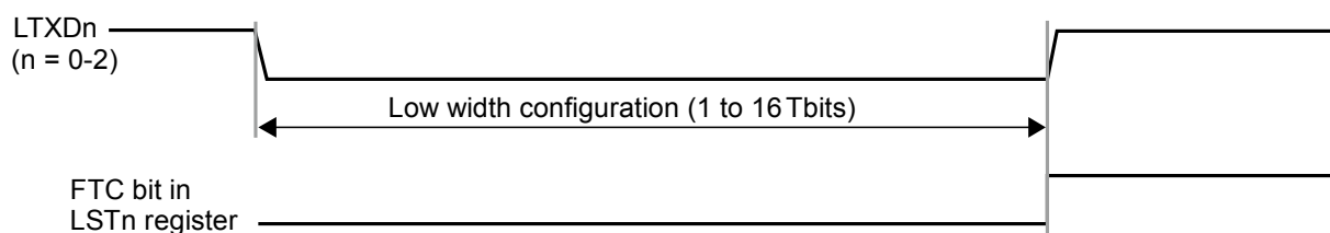
Figure 17-18. Wake-up Transmission Timing
