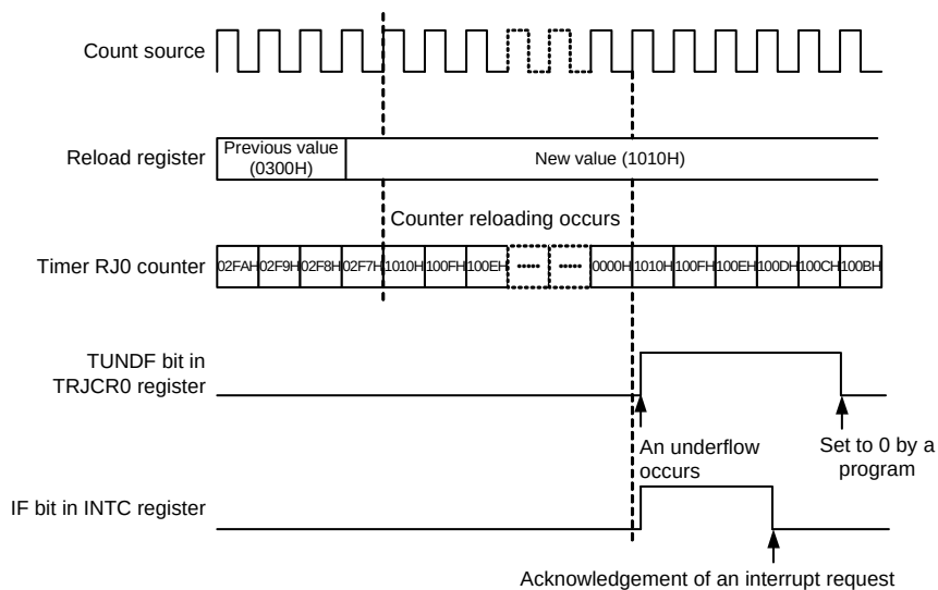
Figure 7-12. Operation Example in Timer Mode
