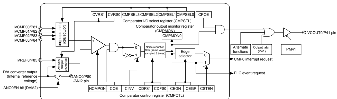
Figure 14-1. Comparator Block Diagram
