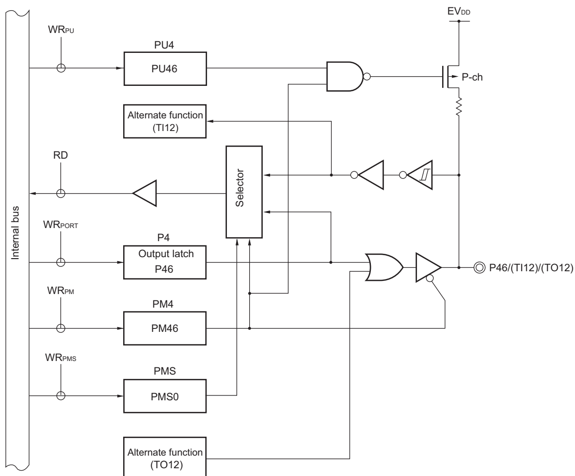
Figure 4-35. Block Diagram of P46
