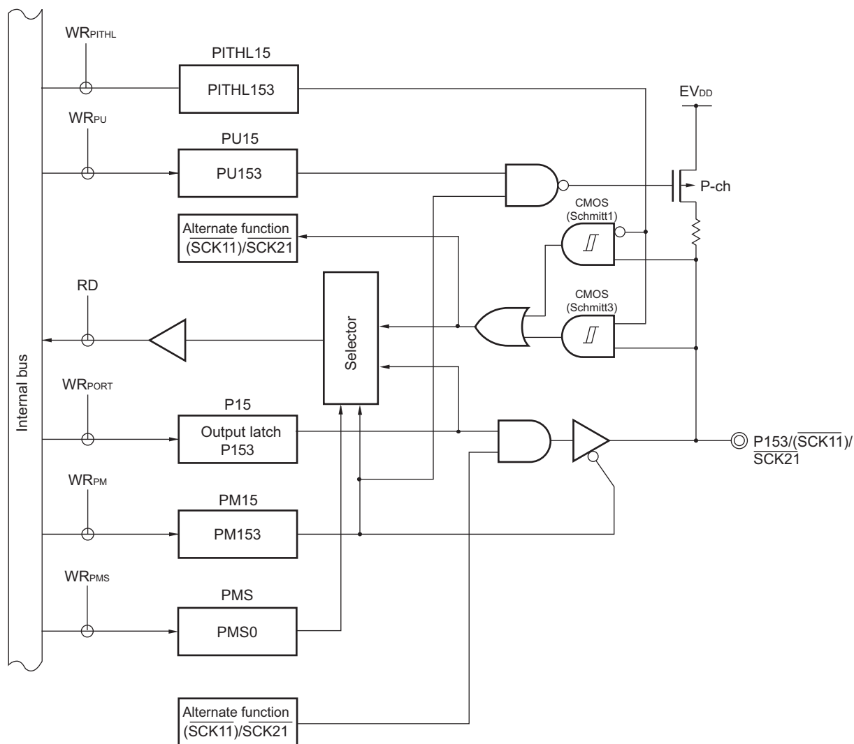
Figure 4-88. Block Diagram of P153
