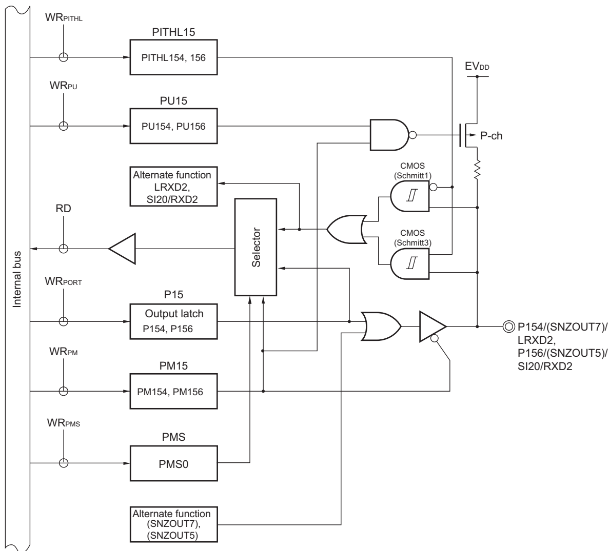
Figure 4-89. Block Diagram of P154, P156
