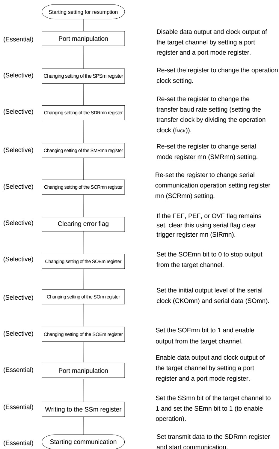
Figure 15-33. Procedure for Resuming Master Transmission (CSI00, CSI01, CSI10, CSI11)
