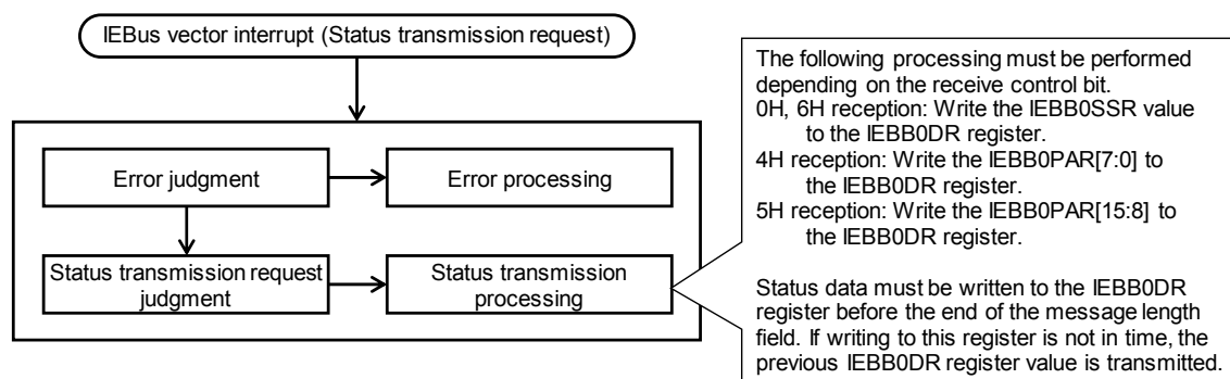
Figure 19-44. IEBus vector interrupt (Status transmission request) processing flow example (Slave transmission)
