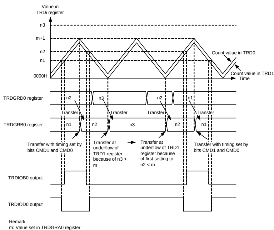
Figure 8-65. Operation When Value in Buffer Register \geq Value in TRDGRA0 Register in Complementary PWM Mode
