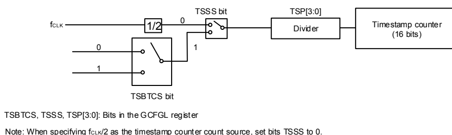
Figure 18-6. Timestamp Function Block Diagram
