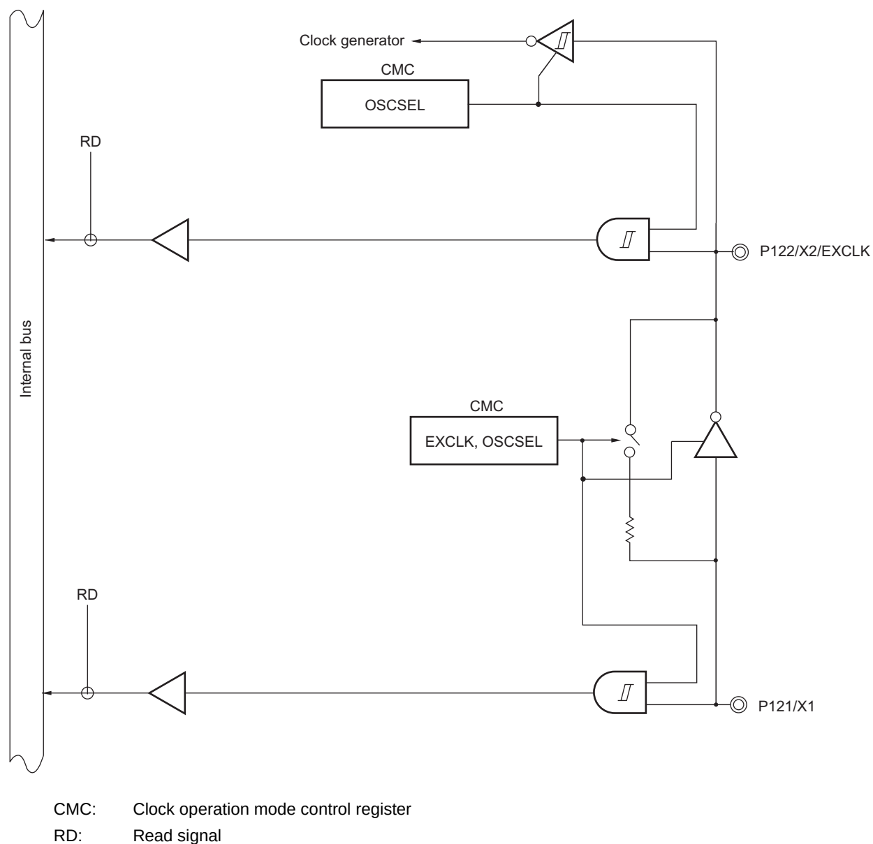
Figure 4-75. Block Diagram of P121 and P122
