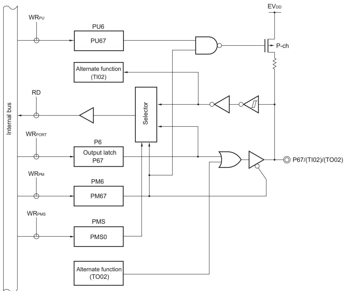
Figure 4-52. Block Diagram of P67
