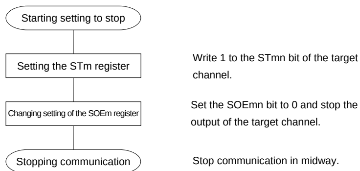
Figure 15-150. Procedure for Stopping Slave Transmission/Reception
