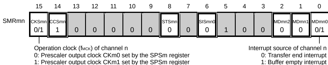
Figure 15-90. Example of Contents of Registers for Slave Transmission/Reception of 3-Wire Serial I/O (CSI00, CSI01, CSI10, CSI11, CSI20, CSI21) (1/2)
