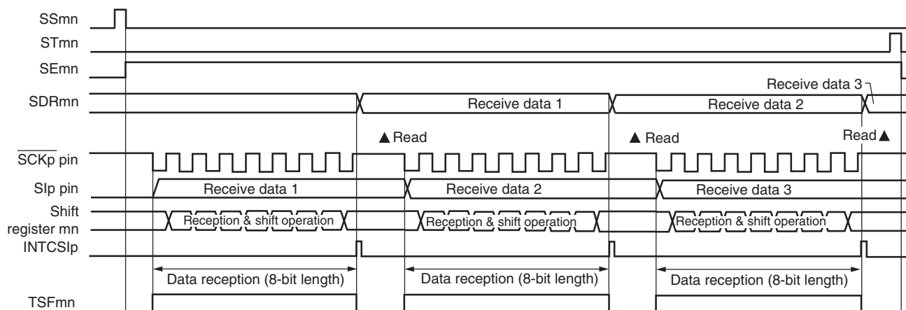
Figure 15-87. Timing Chart of Slave Reception (in Single-Reception Mode)
