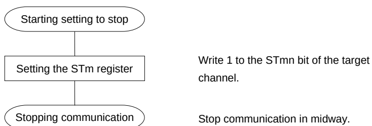
Figure 15-82. Procedure for Stopping Slave Reception (CSI00, CSI01, CSI10, CSI11)
