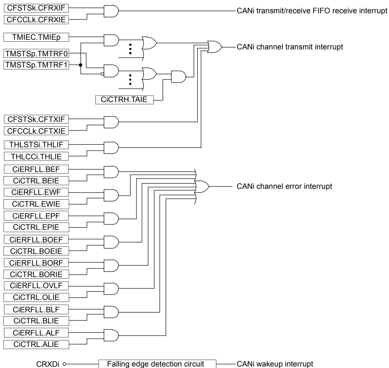
Figure 18-15. CAN Channel Interrupt Block Diagram
