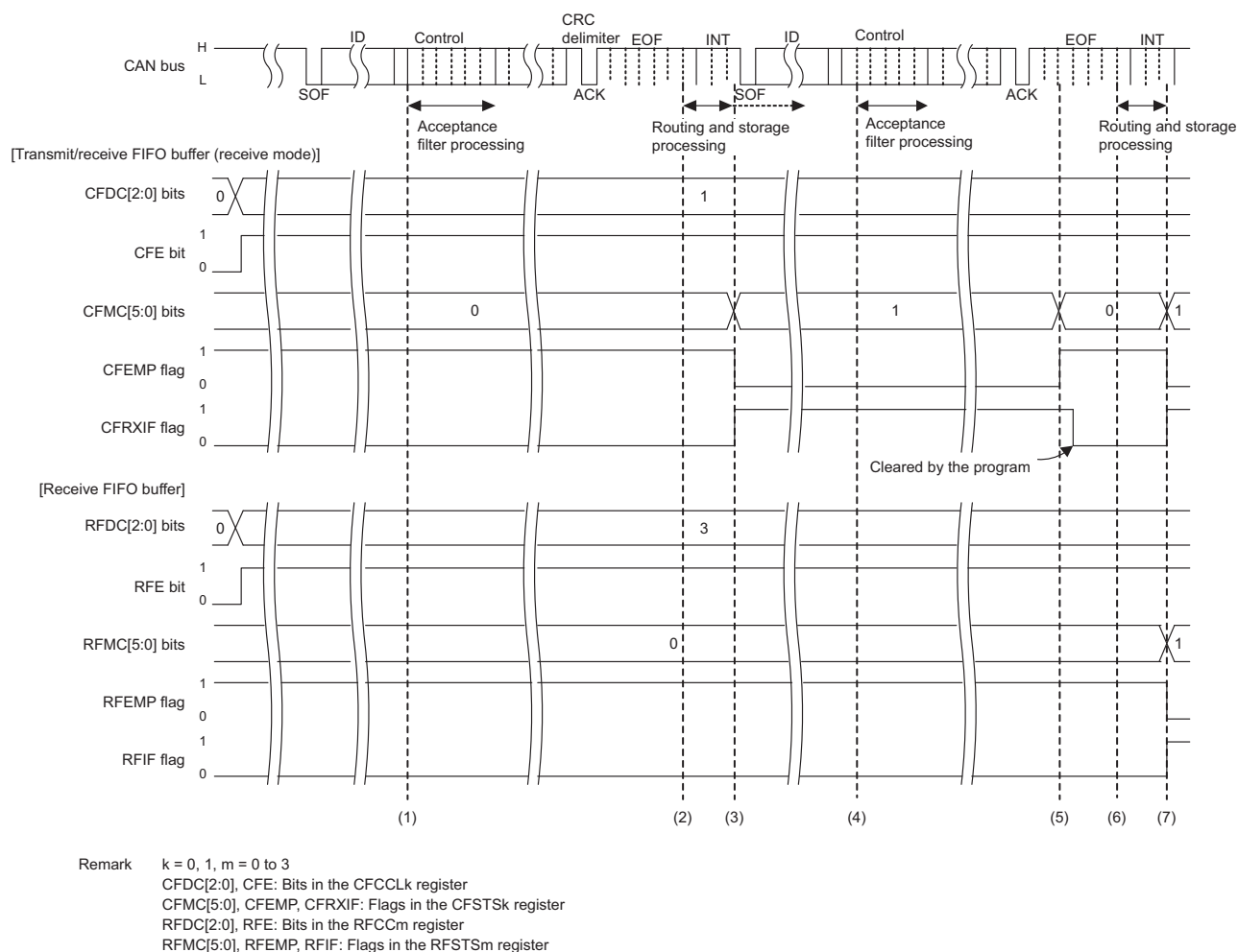
Figure 18-26. FIFO Buffer Reception Timing Chart
