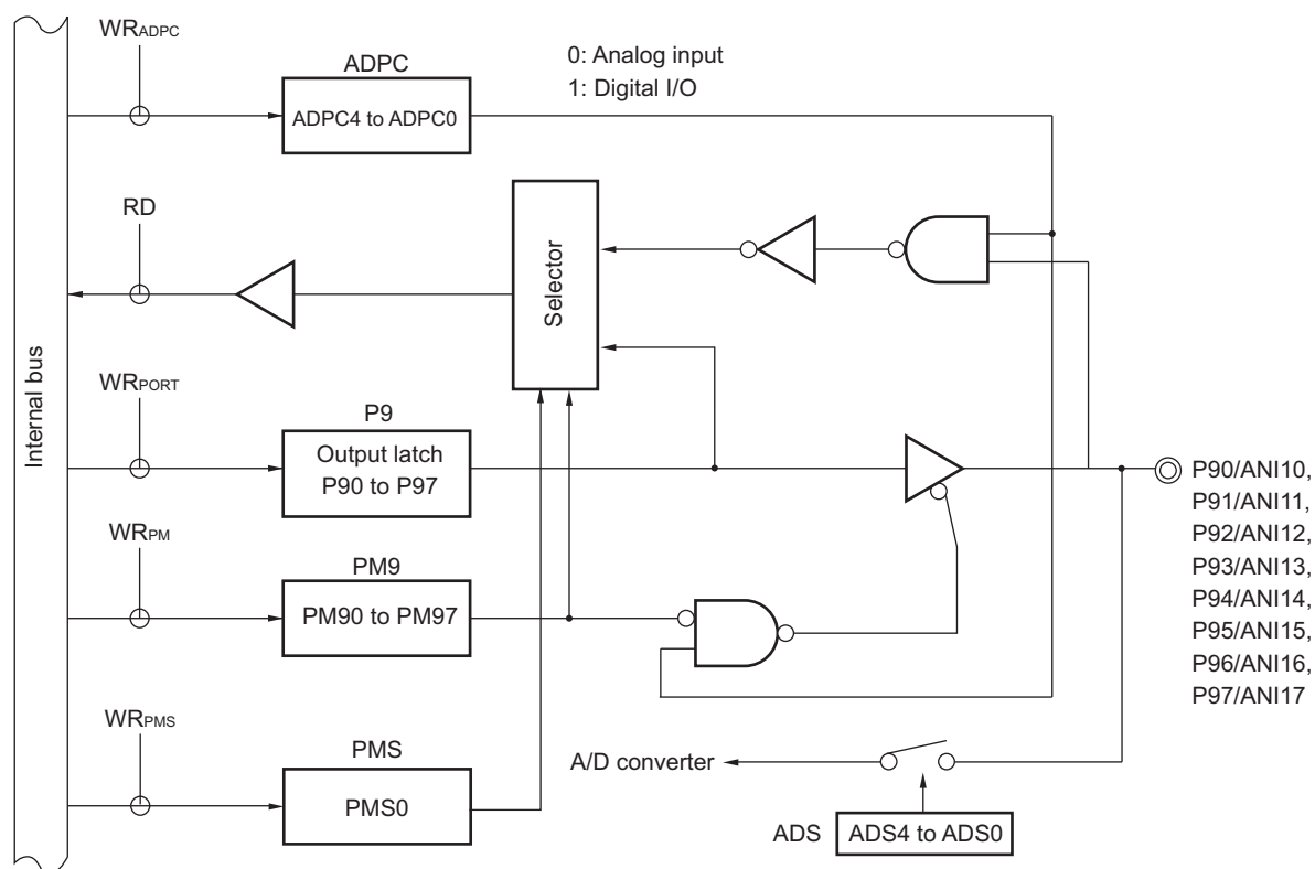
Figure 4-69. Block Diagram of P90 to P97
