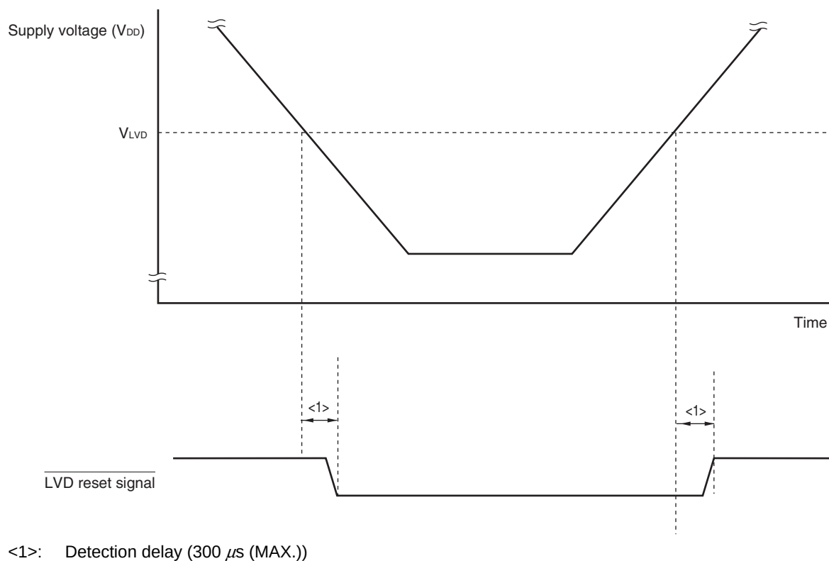
Figure 27-10. Delay from The Time LVD Reset Source Is Generated until The Time LVD Reset Has Been Generated or Released
