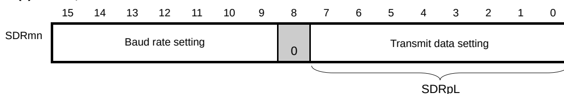
Figure 15-67. Example of Contents of Registers for Slave Transmission of 3-Wire Serial I/O (CSI00, CSI01, CSI10, CSI11, CSI20, CSI21) (2/2)
