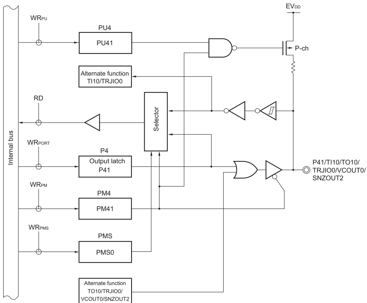
Figure 4-30. Block Diagram of P41
