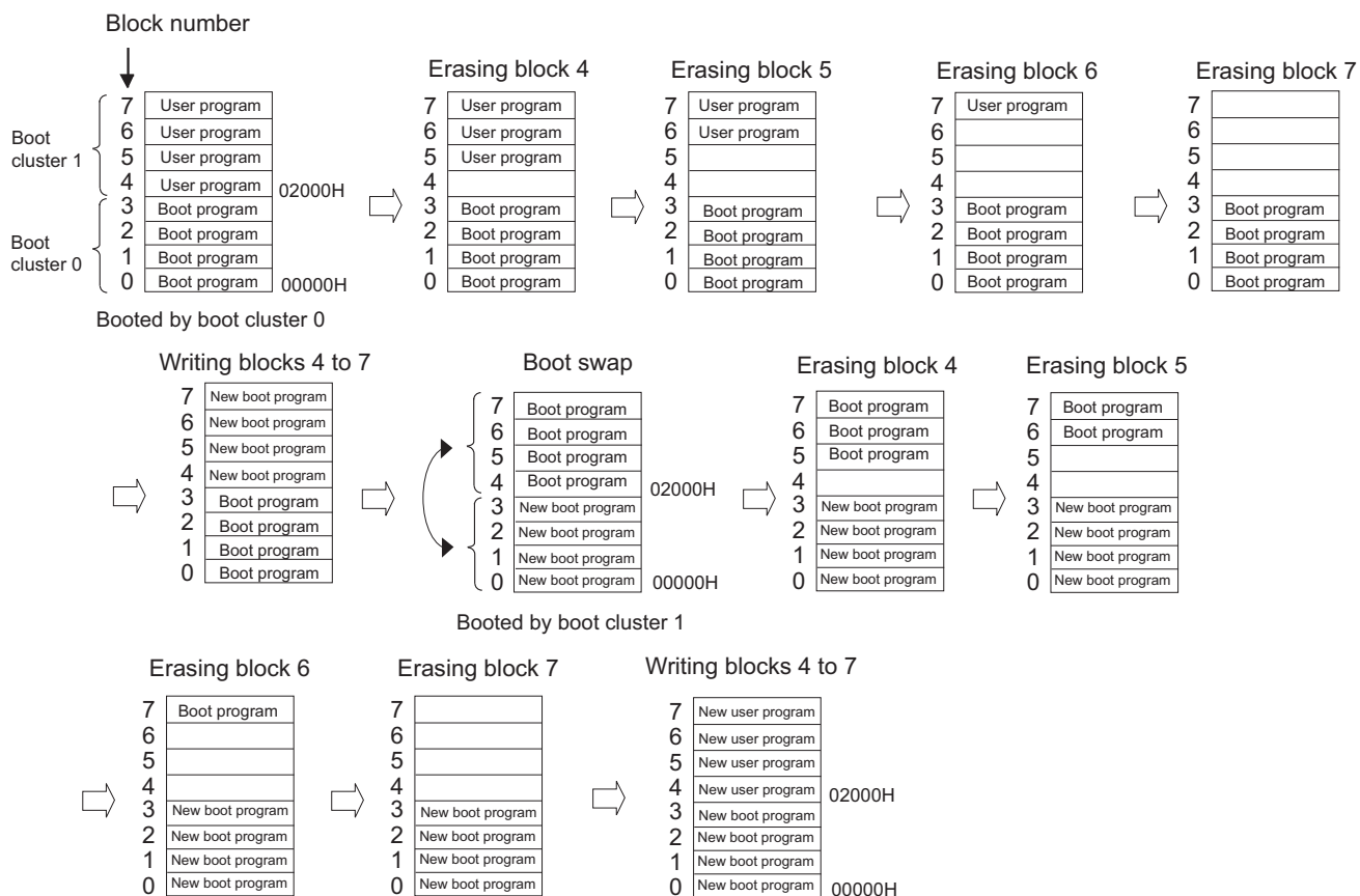
Figure 31-10. Example of Executing Boot Swapping
