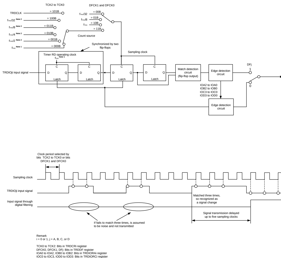
Figure 8-47. Block Diagram of Digital Filter
