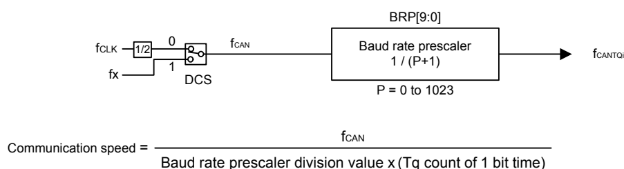
Figure 18-19. CAN Clock Control Block Diagram
