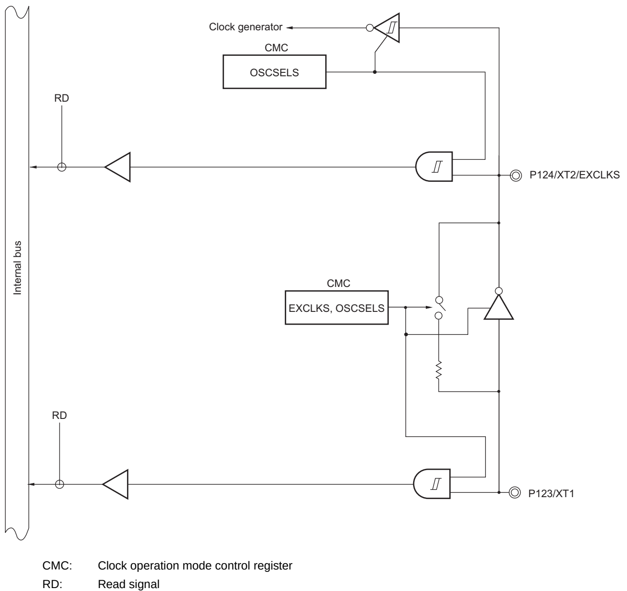
Figure 4-76. Block Diagram of P123 and P124
