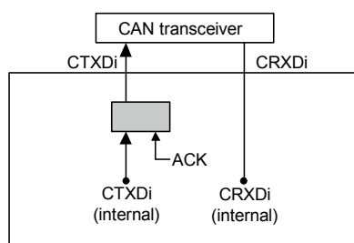
Figure 18-11. Connection when Self-Test Mode 0 is Selected
