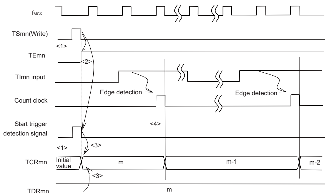
Figure 6-32 Start Timing (In Event Counter Mode)
