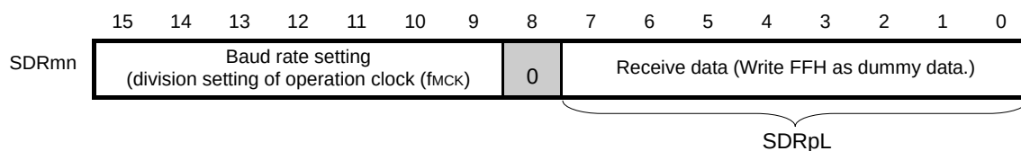
Figure 15-41. Example of Contents of Registers for Master Reception of 3-Wire Serial I/O (CSI00, CSI01, CSI10, CSI11, CSI20, CSI21) (2/2)
