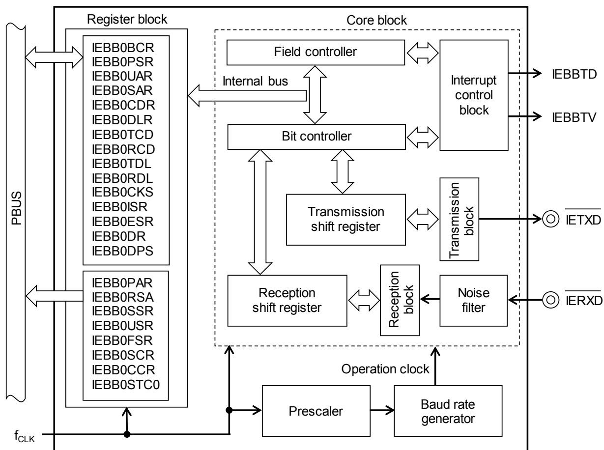
Figure 19-1. IEBB0 block diagram
