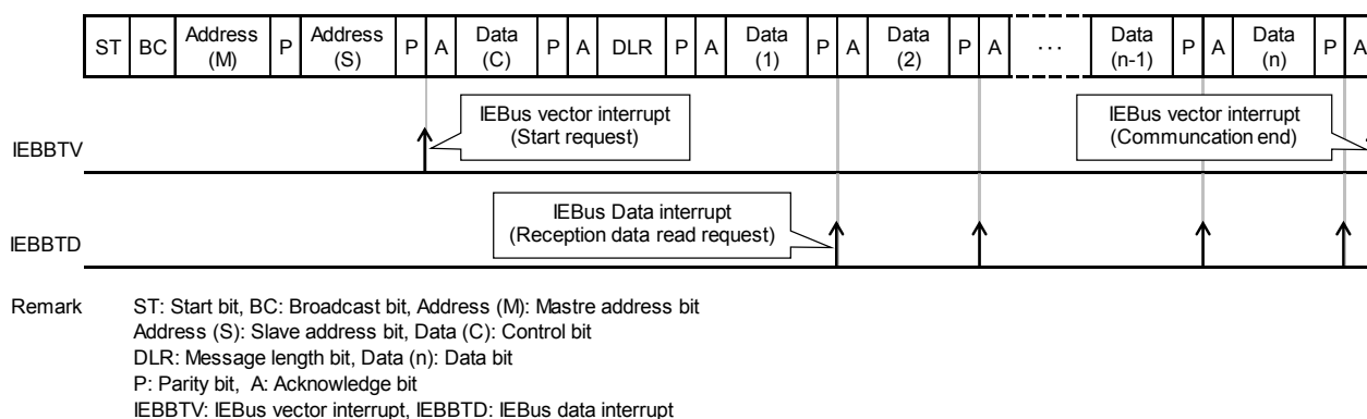
Figure 19-36. Interrupt occurrence timing (Master reception)
