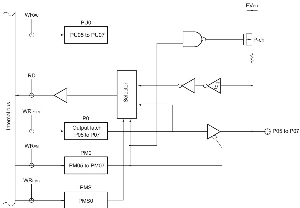
Figure 4-6. Block Diagram of P05 to P07
