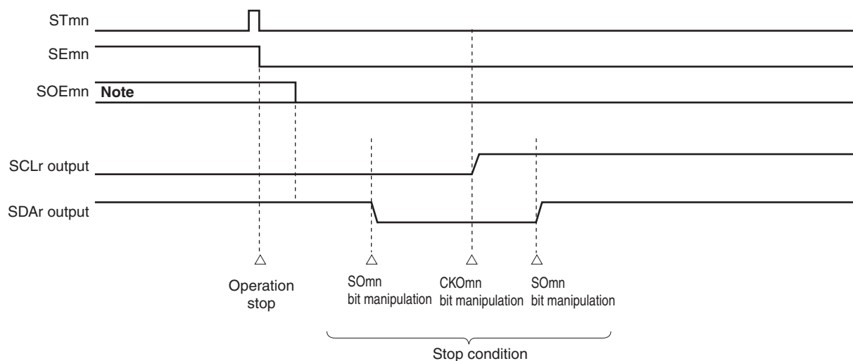
Figure 15-199. Timing Chart of Stop Condition Generation
