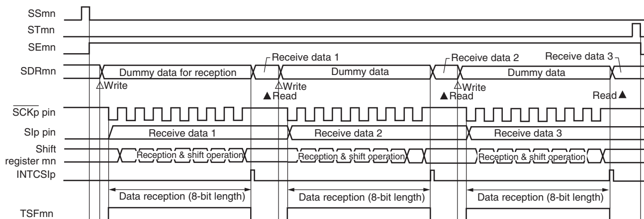
Figure 15-48. Timing Chart of Master Reception (in Single-Reception Mode)
