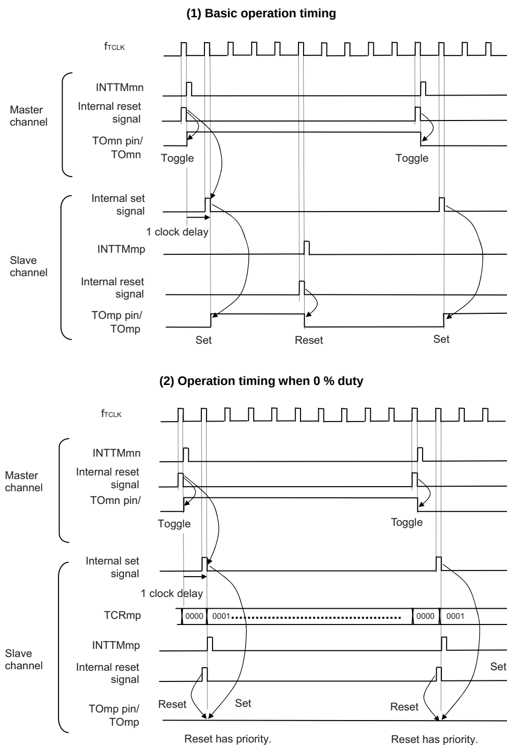
Figure 6-41 Set/Reset Timing Operating Statuses
