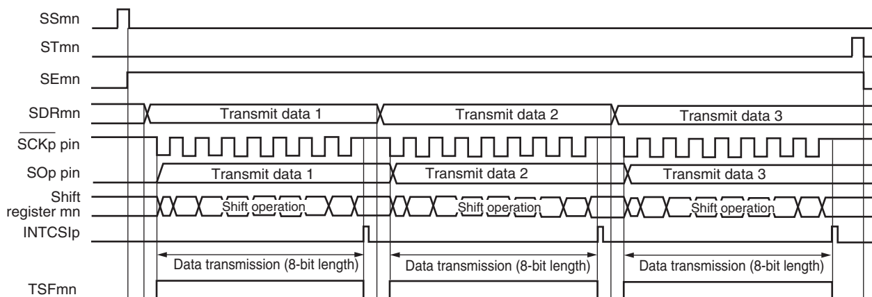
Figure 15-114. Timing Chart of Master Transmission (in Single-Transmission Mode) (Type 1: DAPmn = 0, CKPmn = 0)
