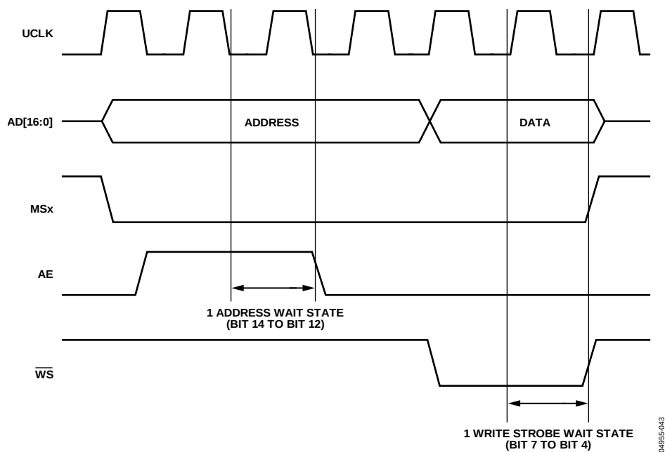
Figure 86. External Memory Write Cycle with Wait States
