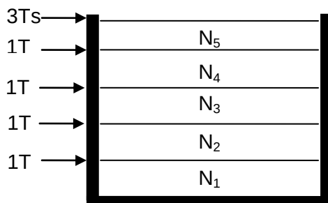
Figure 5 – Winding Diagram
