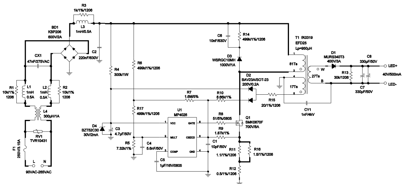
Figure 1 - Schematic
