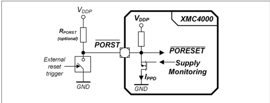
Figure 25 PORST Circuit
