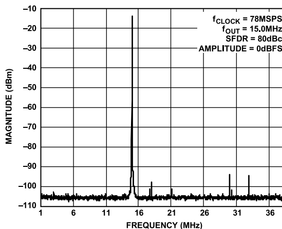
Figure 24. Single-Tone SFDR
