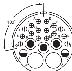
100° Rotation of 32-6
