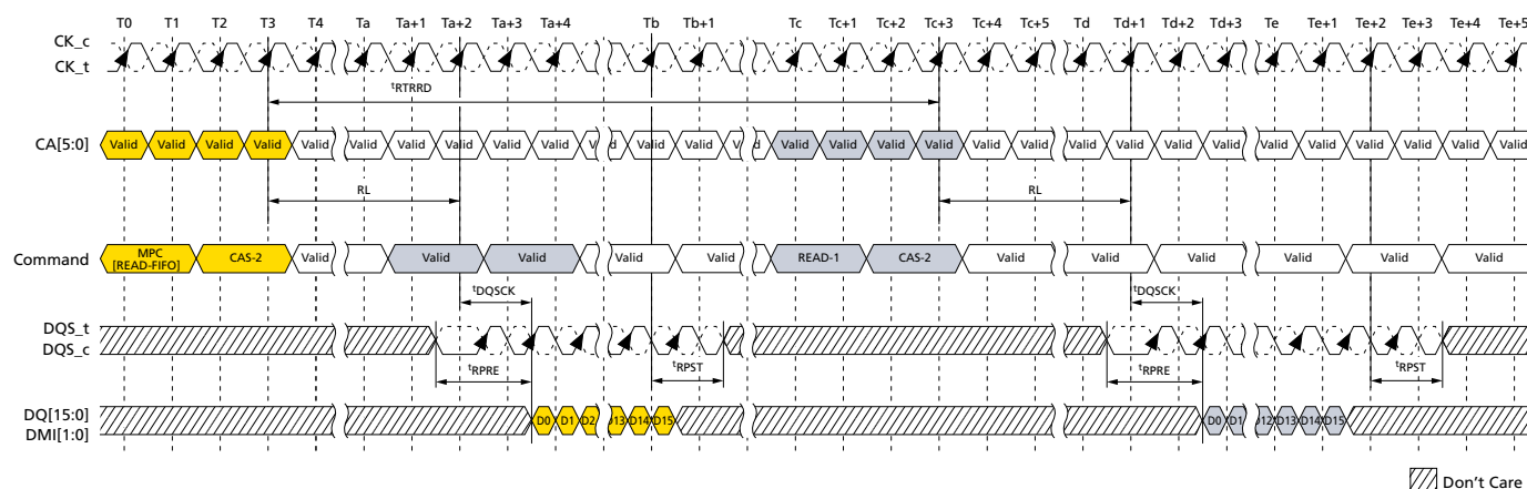
Figure 122: READ-FIFO – t_{\text{RPRE}} = Toggling, t_{\text{RPST}} = 1.5n\text{CK}
