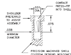
#11 CONTACT FOR .015"-.020" DIAMETER PINS ( \delta = .003 ) 3-FINGER, GROUP A (See page 248)
