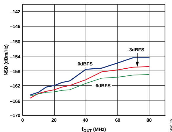
Figure 28. AD9779A Noise Spectral Density vs. f_{OUT} , Digital Full-Scale Over Output Frequency of Single-Tone Input, 2× Interpolation, f_{DATA} = 200 MSPS
