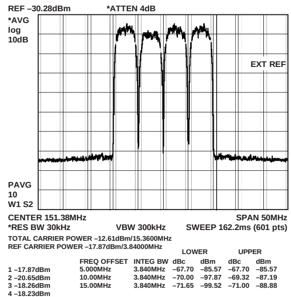
Figure 35. AD9779A Multicarrier W-CDMA Signal, 4x Interpolation, f_{DATA} = 122.88 MSPS, f_{DAC}/4 Modulation
